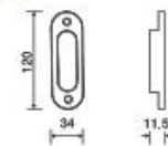
OV-3 Passage Function with no door edge finger pull
