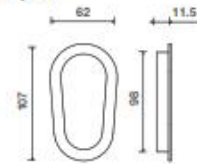
TD-3 Passage Function with no door edge finger pull
