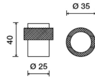
DS545 Barrel
